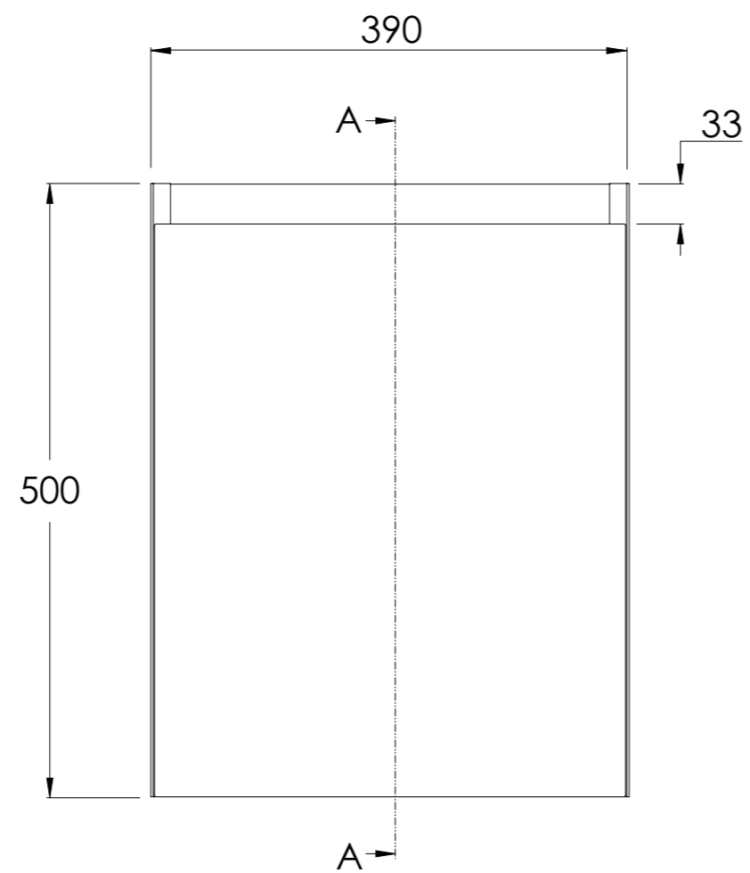
FRONT VIEW
