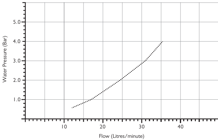
Spout Only
