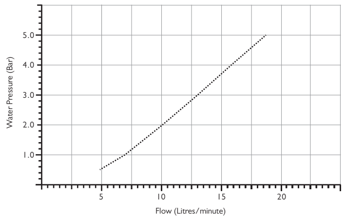
Handshower Only
