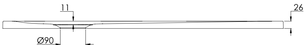
SECTION: A-A
